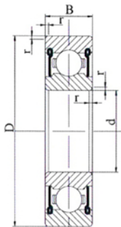
Shield(Z)
