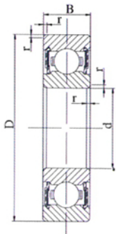
Seal(RS)
