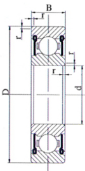
Shield(Z)
